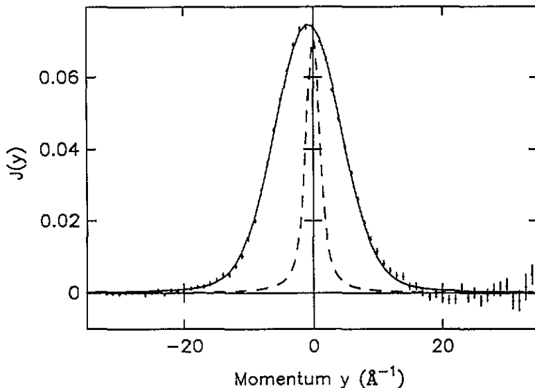
Figure 4. Compton profile J_M^a(y_M) for hydrogen in a-C:H, obtained by combining all forward angle data sets as described in equation (13). The solid line is the fit described in the text; the dotted line is the instrument resolution function.
