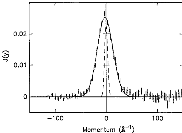
Figure 7. Compton profile J_M^a(y_M) for carbon obtained from the diamond sample by using the 6671 meV uranium resonance as described in the text. The solid line is the fit, the dotted line the resolution function.
