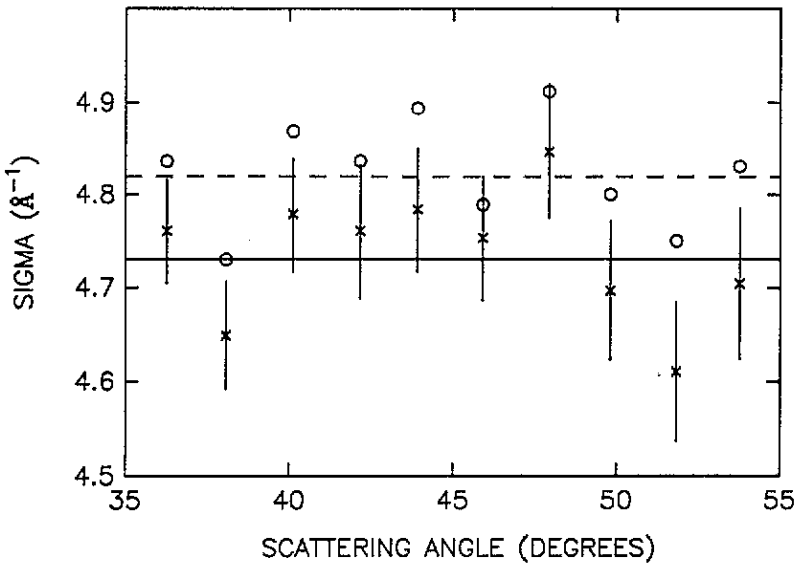
Figure 5. Values of \sigma_M^\theta ( \times ) and \sigma_{MS}^\theta ( \circ ) derived from fits to data sets obtained at different scattering angles. Within statistical error no systematic variation with scattering angle is observed. The mean values of \bar{\sigma}_M^\theta (solid line) and \bar{\sigma}_{MS}^\theta (dashed line) are also shown.
