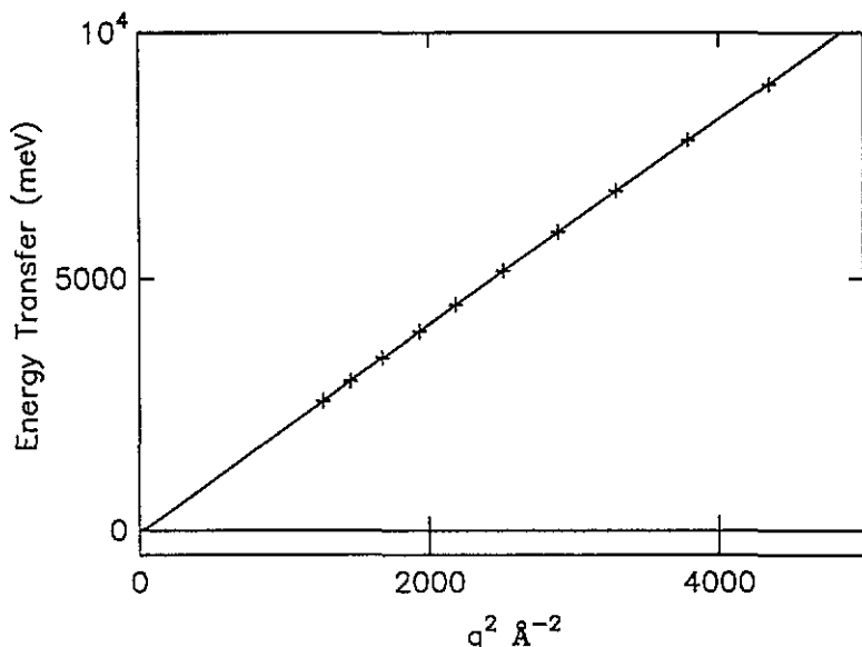
Figure 8. Experimental values of \bar{\omega}_M as a function of \bar{q}_M^2 for the hydrogen atom in a-C:H. The error bars are too small to be seen. The solid line is a fit to equation (14).
